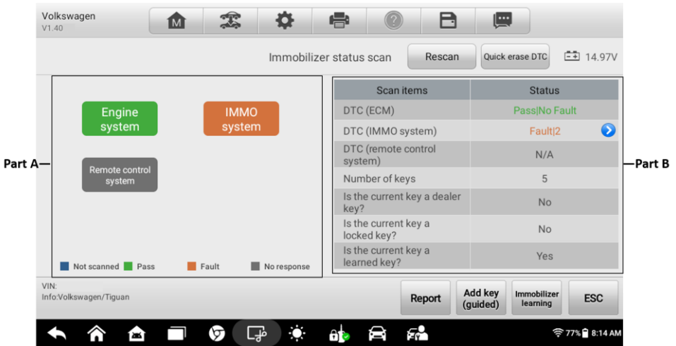
Figure 4-7 Main Section of IMMO Status Scan
